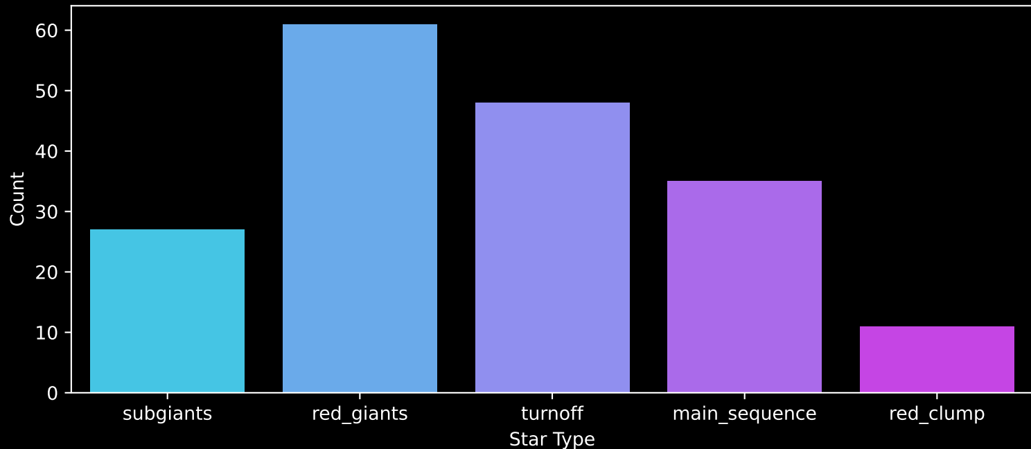
APOGEE DR17 Field: [CVZ_OB05_btx] Count plot of Star Type
