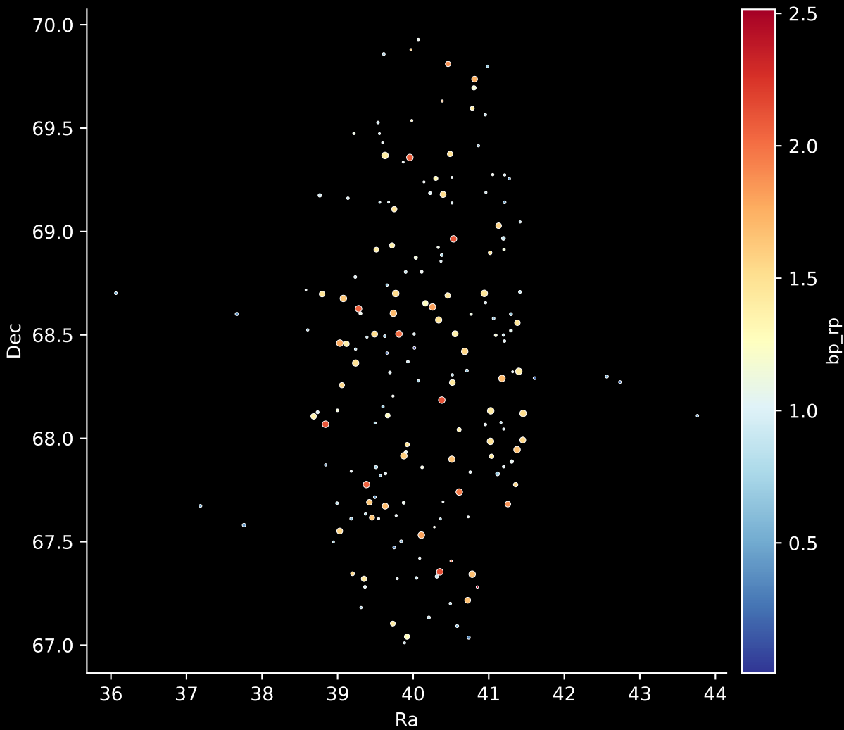
APOGEE DR17 Field: [CVZ_OB05_btx] Stars: 182
