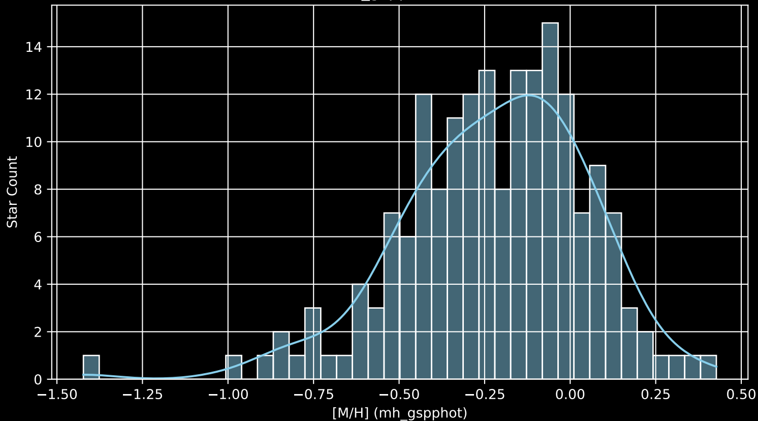
APOGEE DR17 Field: [CVZ_OB05_btx [M/H] (mh_gspphot) (n= 180)
