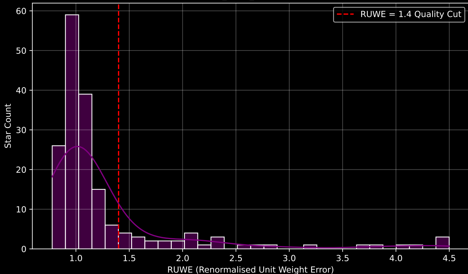
GAPOGEE DR17 Field [CVZ_OB05_btx] RUWE Distribution (n= 177)
