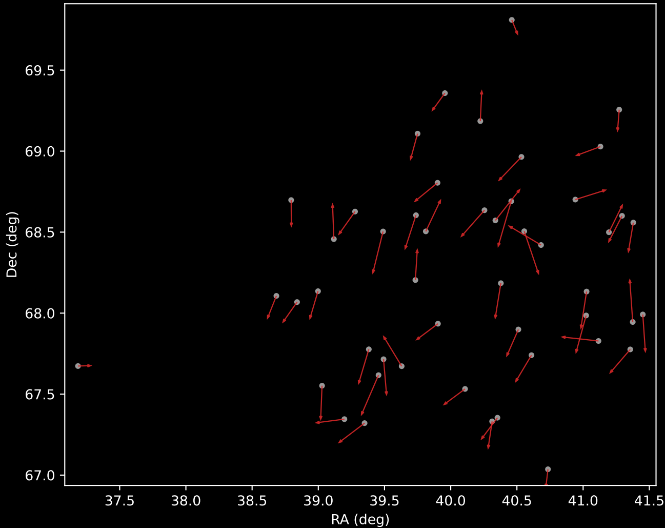
APOGEE DR17 Cluster 6 Proper Motion Vectors (n=49)
