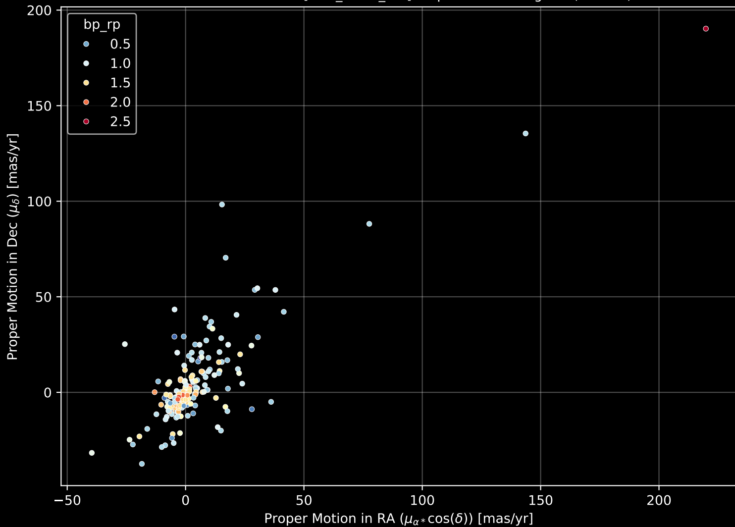
APOGEE DR17 Field: [CVZ_OB05_btx] Proper Motion Diagram (n= 182)
