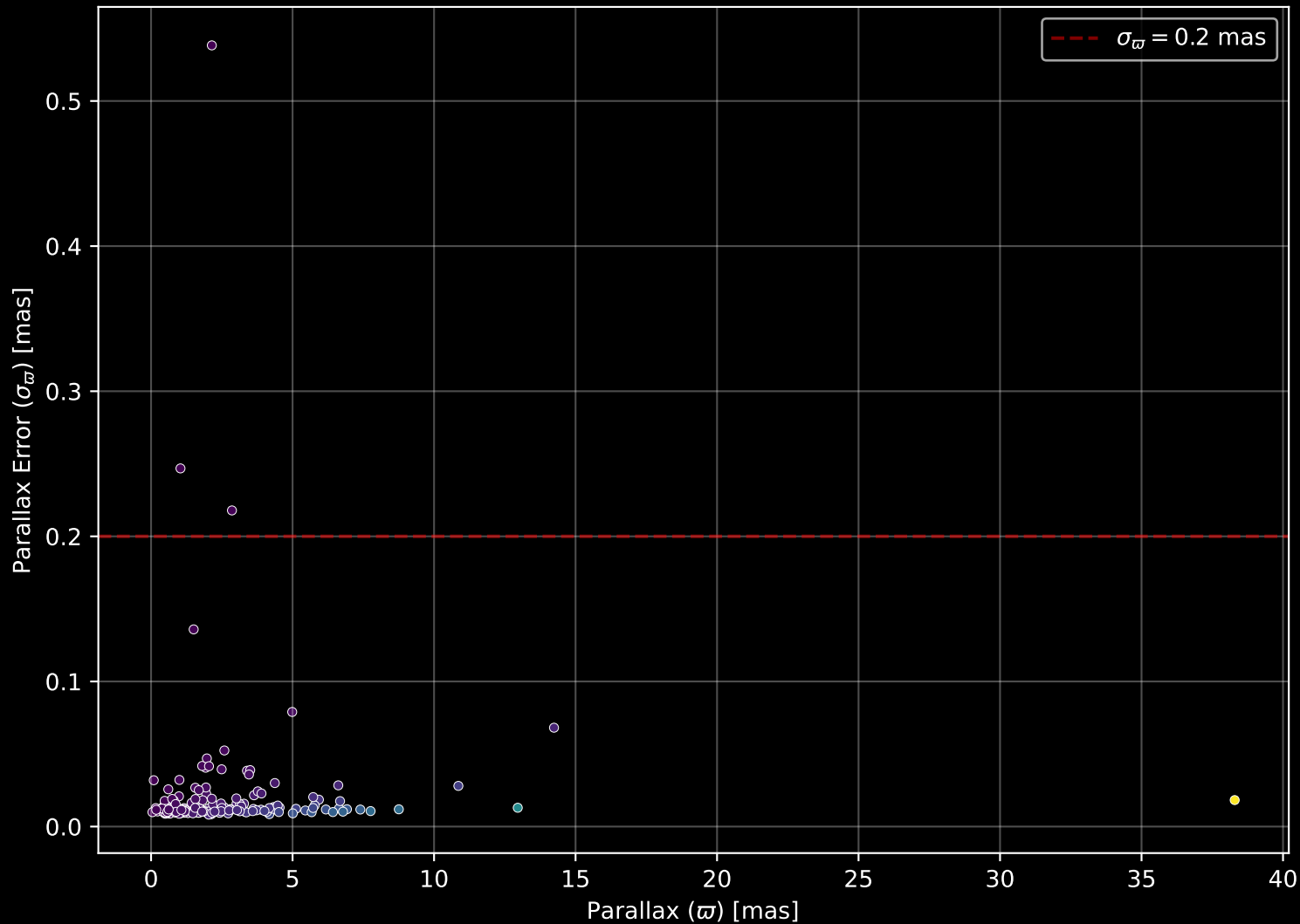
APOGEE DR17 Field: [CVZ_OB05_btx] Parallax Quality (n= 182)
